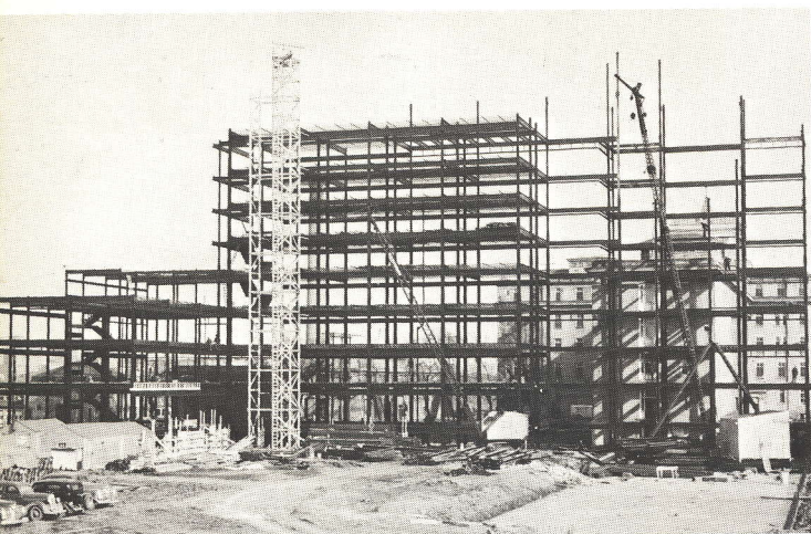
Steel framework of the half completed eight storey addition to St. Boniface Hospital.
